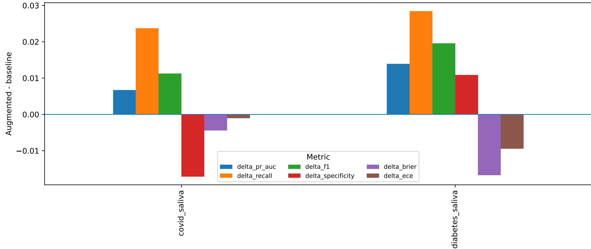
Saliva datasets: mean effect of train-only augmentation
