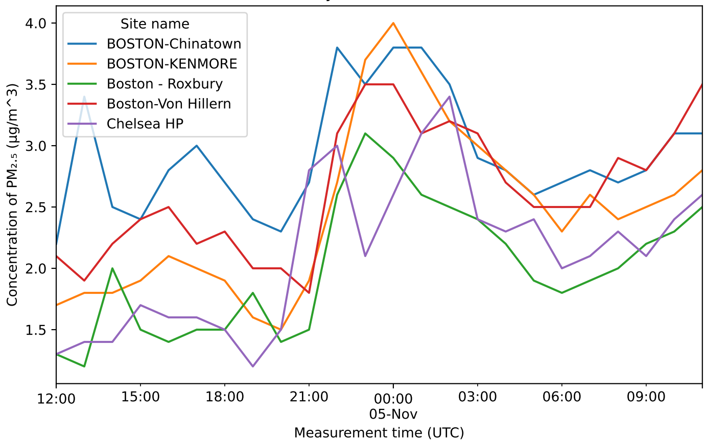
PM 2.5 concentration by station as of November 05, 2025
