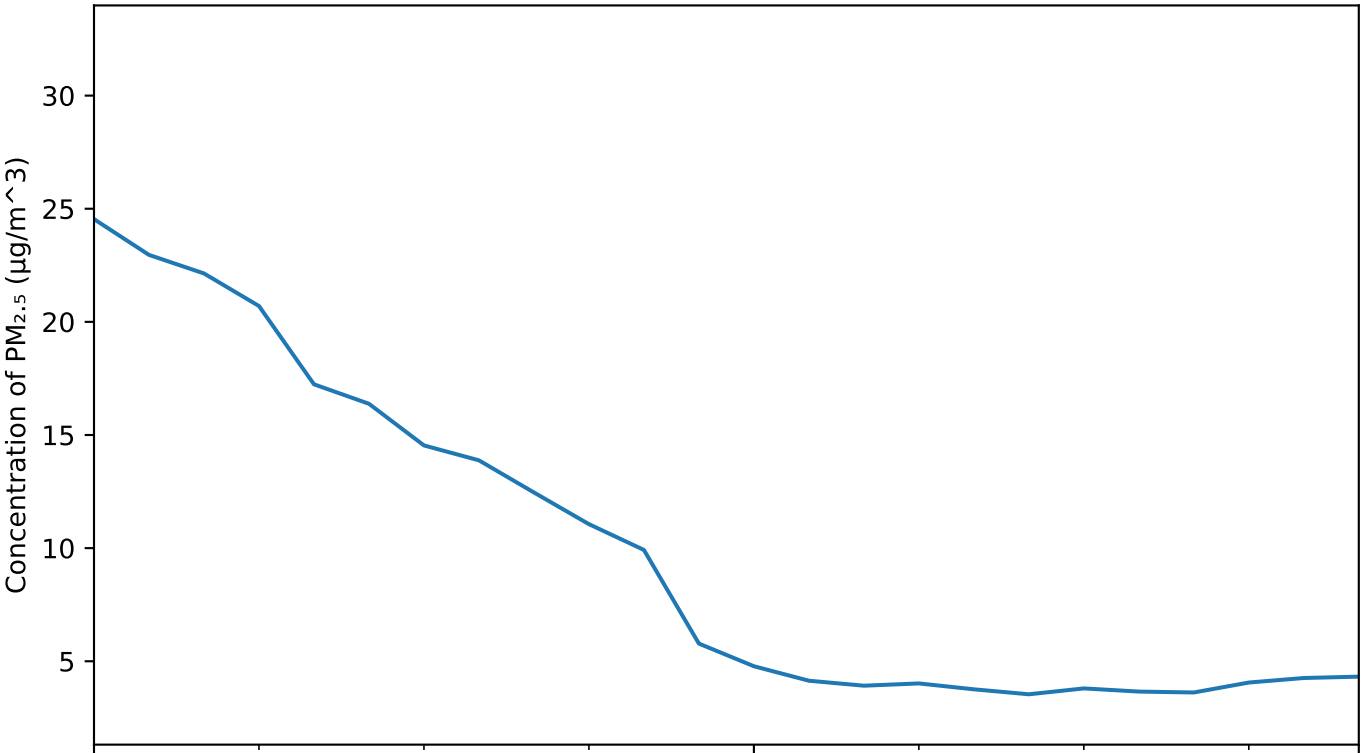
Average PM 2.5 concentration as of November 23, 2025
