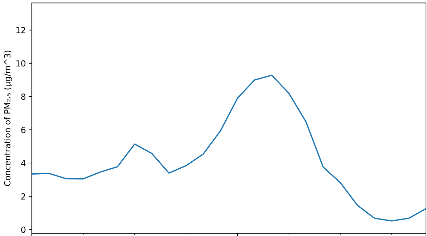
Average PM 2.5 concentration as of November 06, 2025
