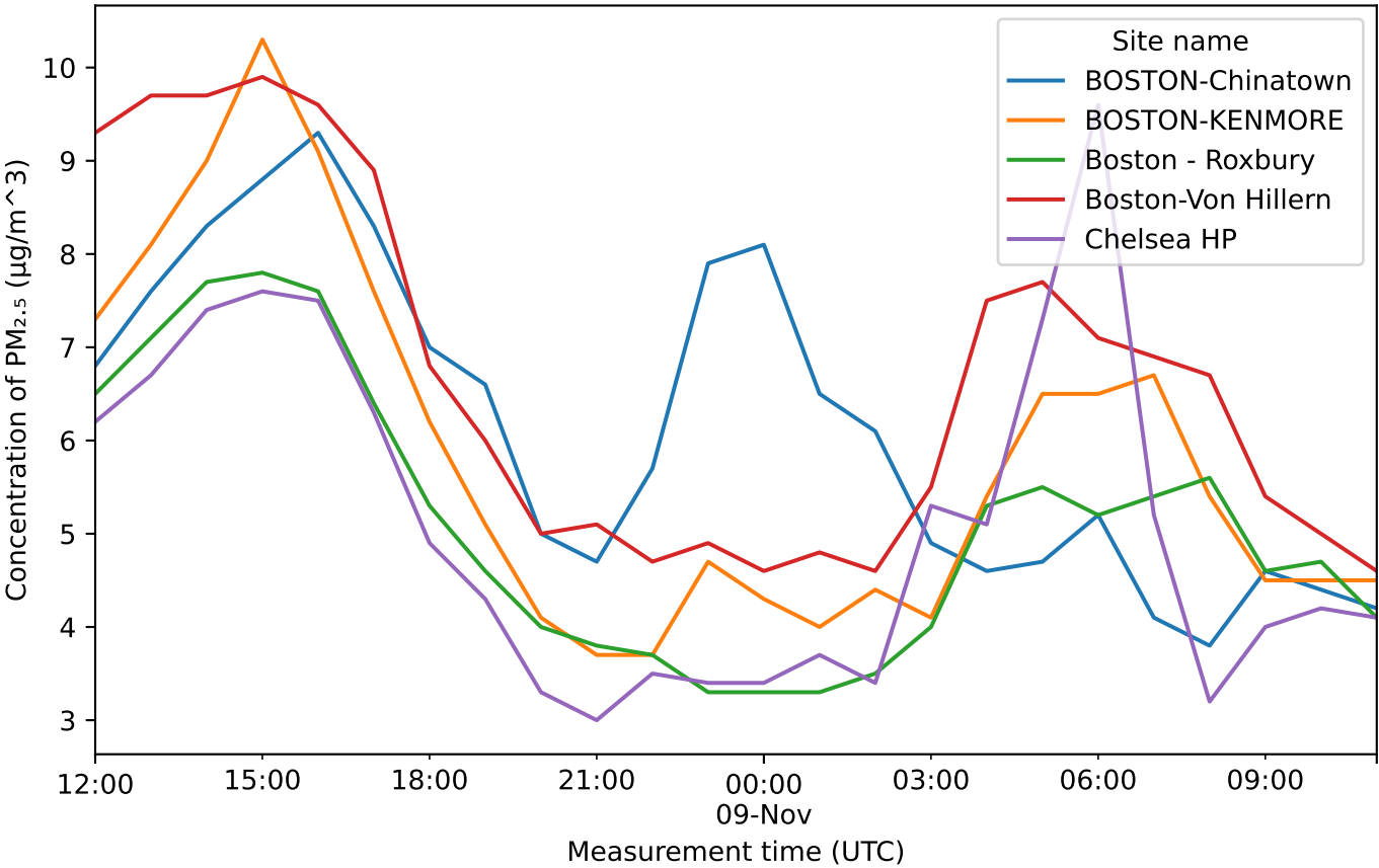
PM 2.5 concentration by station as of November 09, 2025
