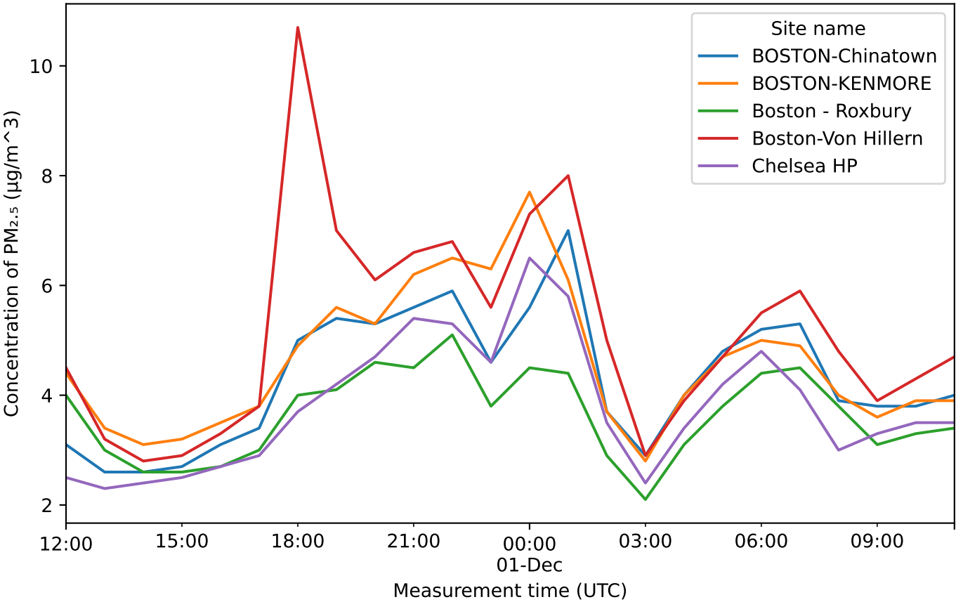
PM 2.5 concentration by station as of December 01, 2025
