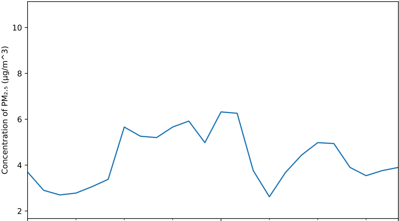
Average PM 2.5 concentration as of December 01, 2025
