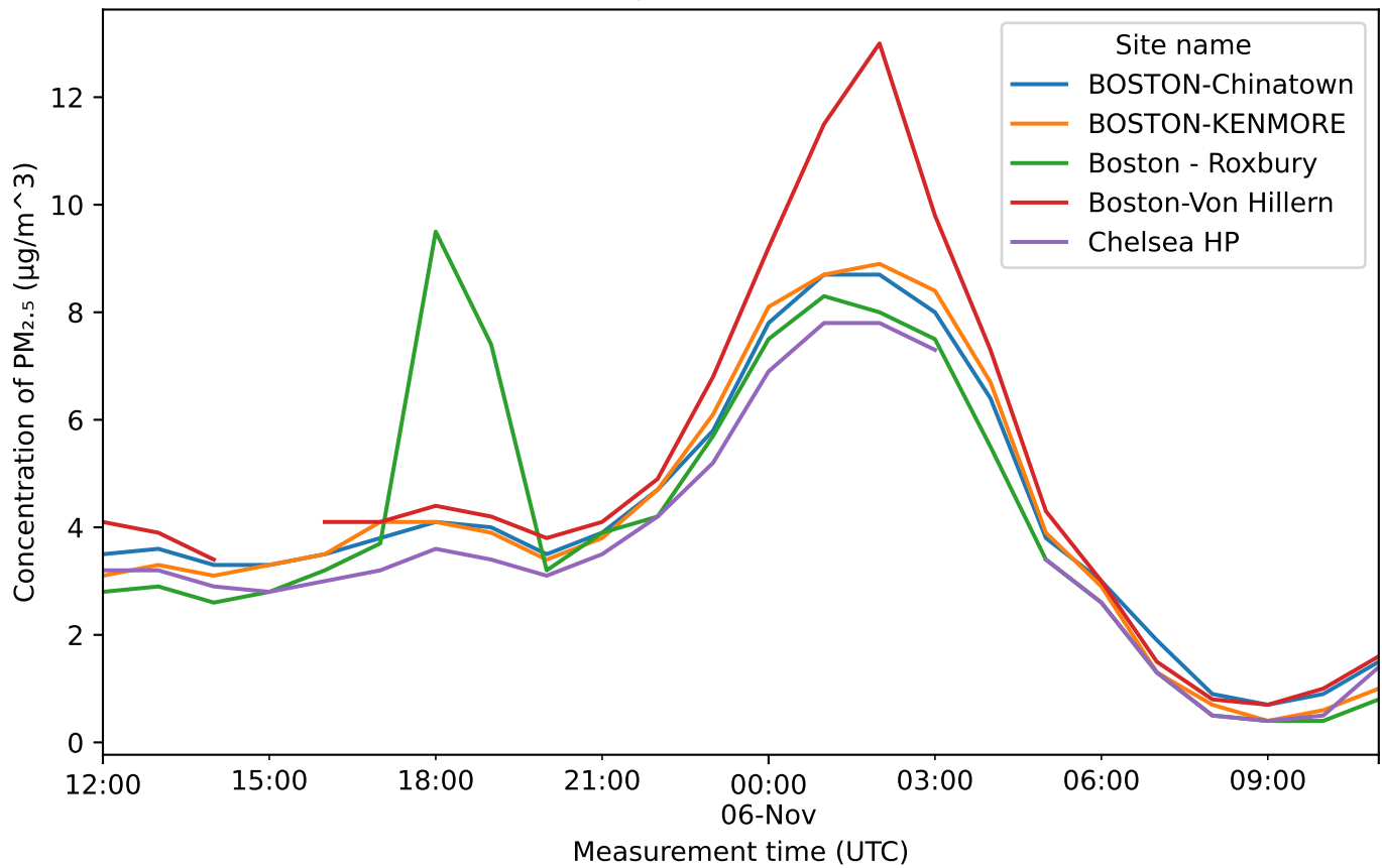
PM 2.5 concentration by station as of November 06, 2025
