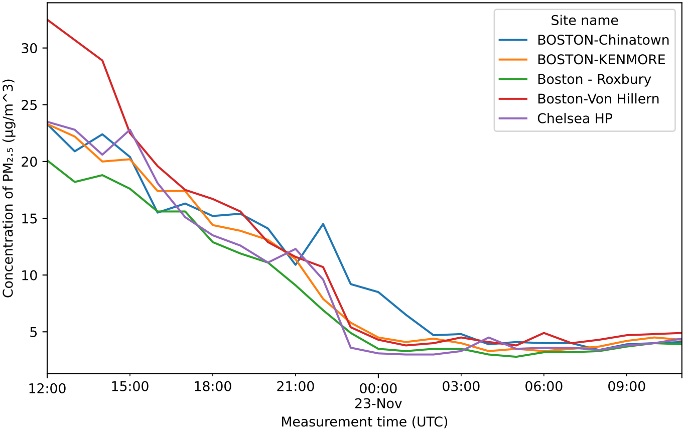
PM 2.5 concentration by station as of November 23, 2025
