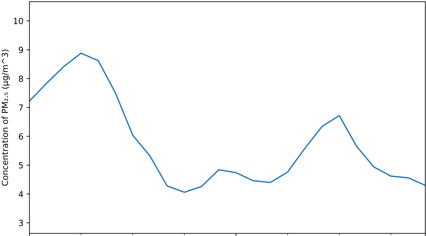
Average PM 2.5 concentration as of November 09, 2025
