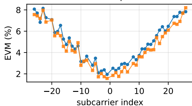
constellation error per subcarrier
