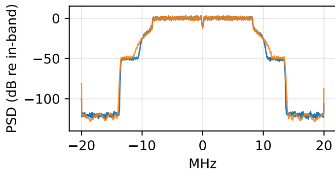
PSD - full burst
