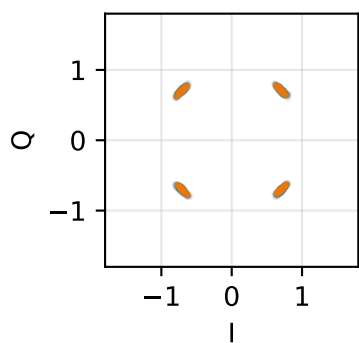
constellation, validated RX, pilot-tracked real 5.27% recon 4.91%
