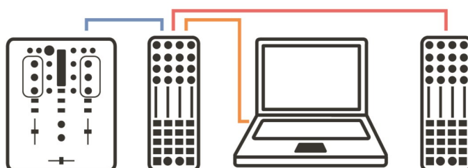
AUDIO MIXER + K1 + K2 CONTROLLER via X:LINK + LAPTOP via USB
