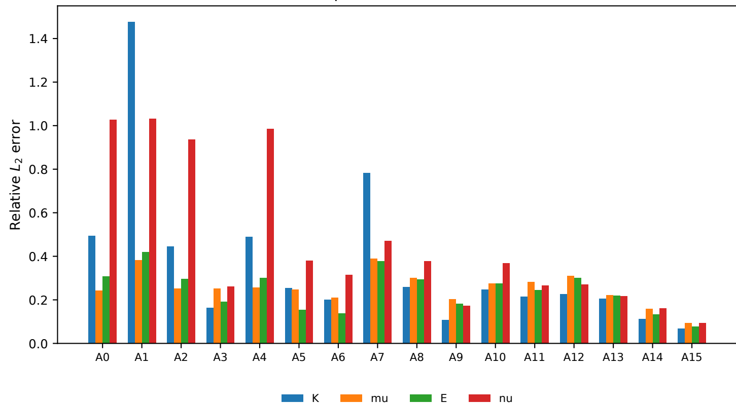
Material-parameter inversion error
