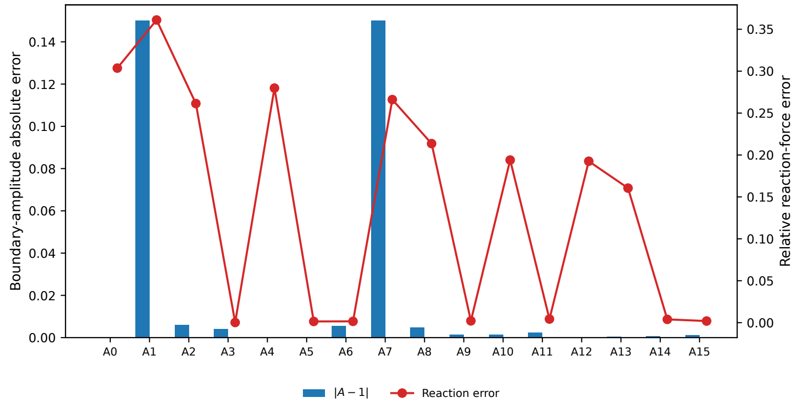
Boundary-amplitude and reaction-force errors
