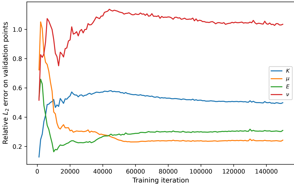
Material-parameter error evolution
