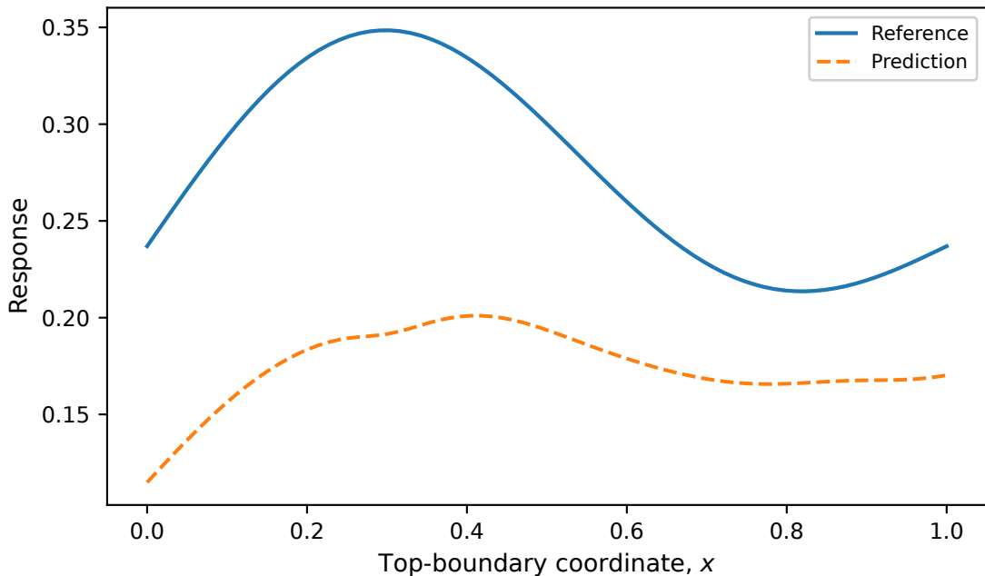
Top-boundary reaction density from constitutive stress
