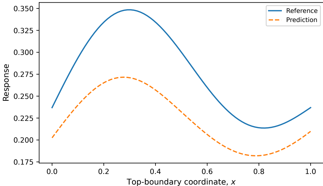
Top-boundary reaction density from constitutive stress
