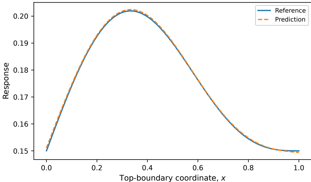
Top-boundary vertical displacement
