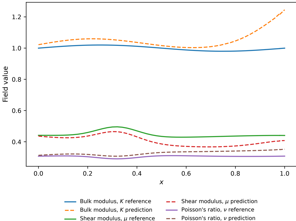
Line-slice comparison at y = 0.75
