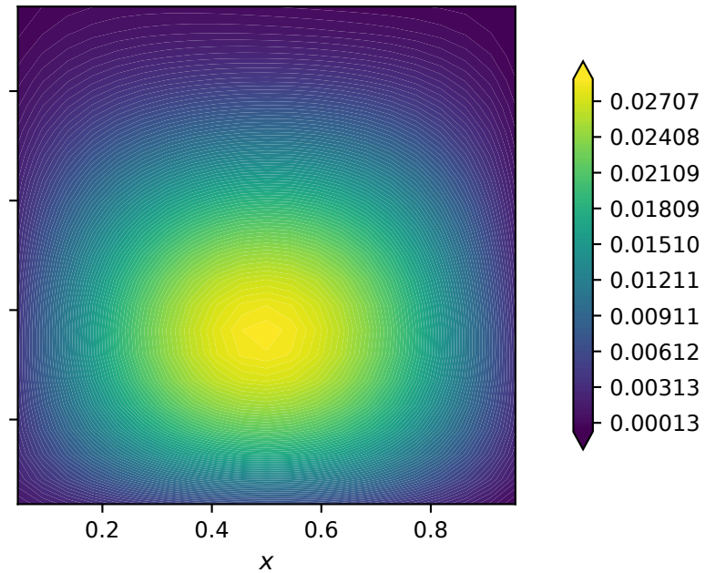
Horizontal displacement, u_x Prediction
