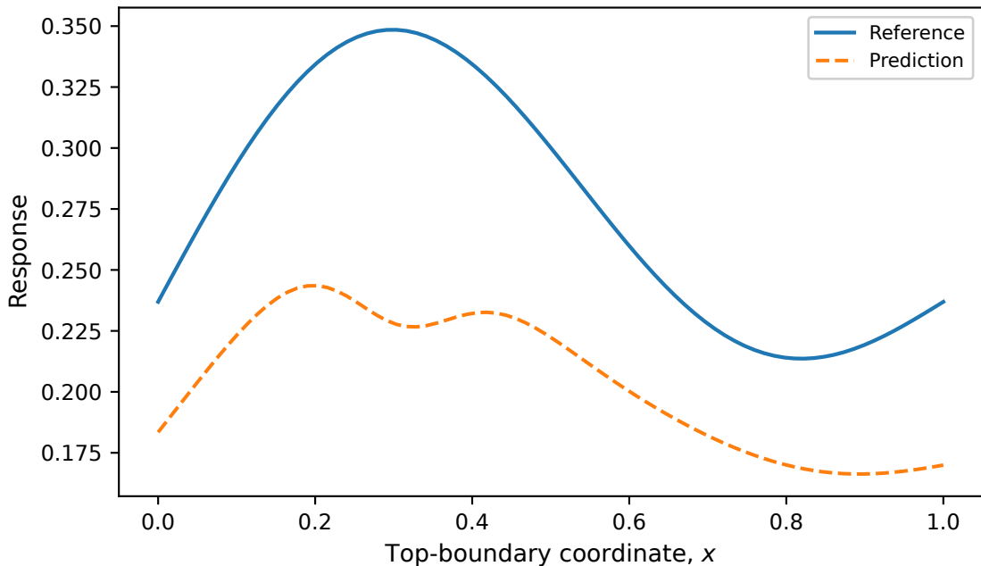
Top-boundary reaction density from stress branch
