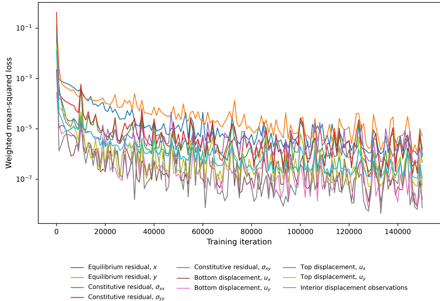
Individual loss components
