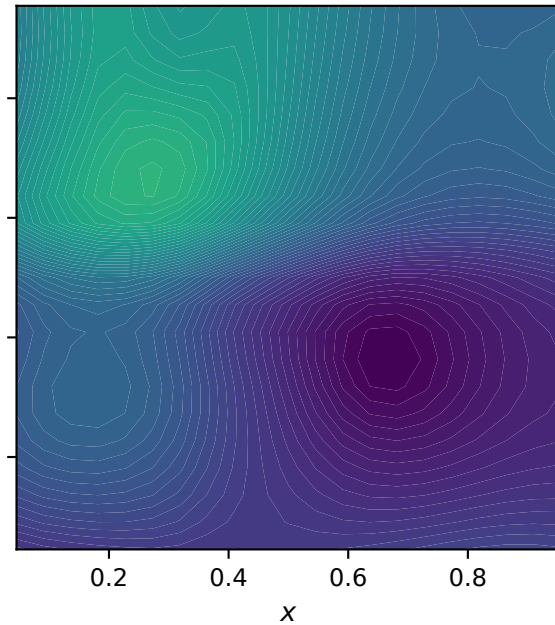
Prediction
