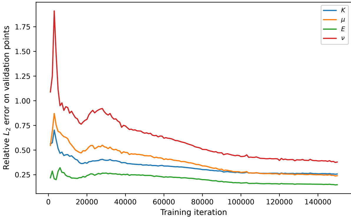
Material-parameter error evolution
