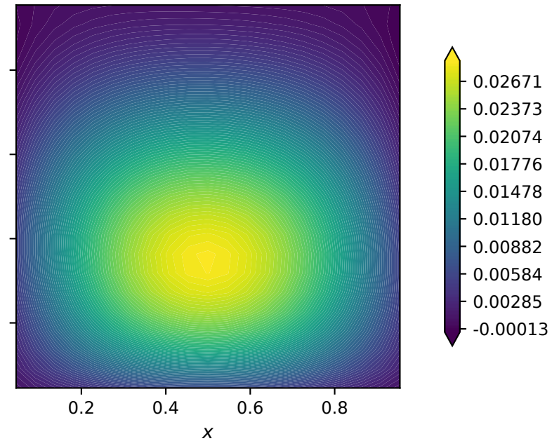
Horizontal displacement, u_x Prediction
