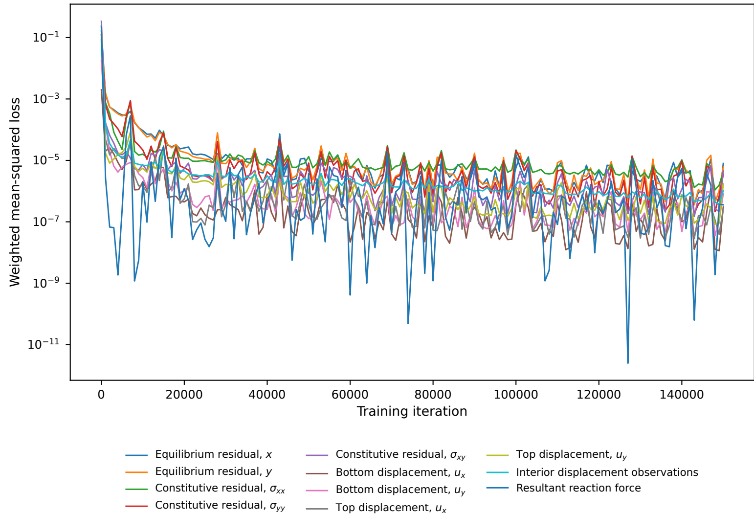
Individual loss components
