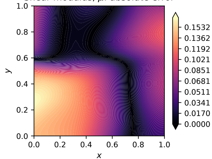
Shear modulus, \mu : absolute error
