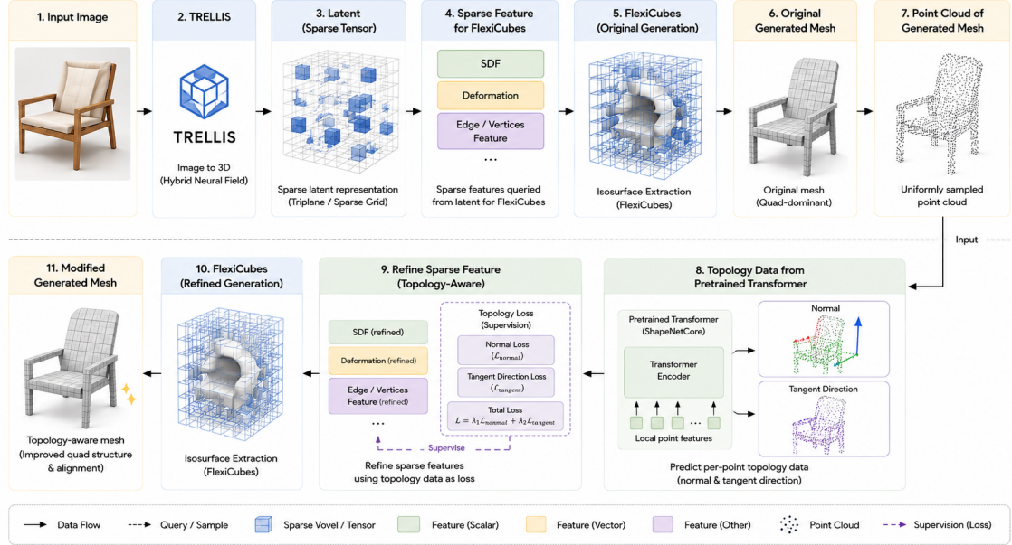
Figure 3.1: Overview of the proposed topology-aware mesh generation framework. An input image is processed by TRELLIS to produce a sparse tensor representation, which is decoded by FlexiCubes to generate an initial mesh. A point cloud sampled from the generated mesh is analyzed by a pretrained Transformer to predict surface normals and tangent directions. These predictions are used as topology supervision during the optimization of the sparse features, resulting in a topology-aware mesh with improved edge-flow while preserving geometric fidelity.
