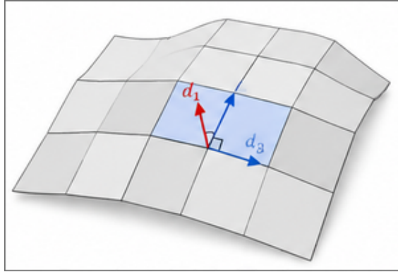
Figure 3.3: Principal direction of a quadrilateral mesh.
