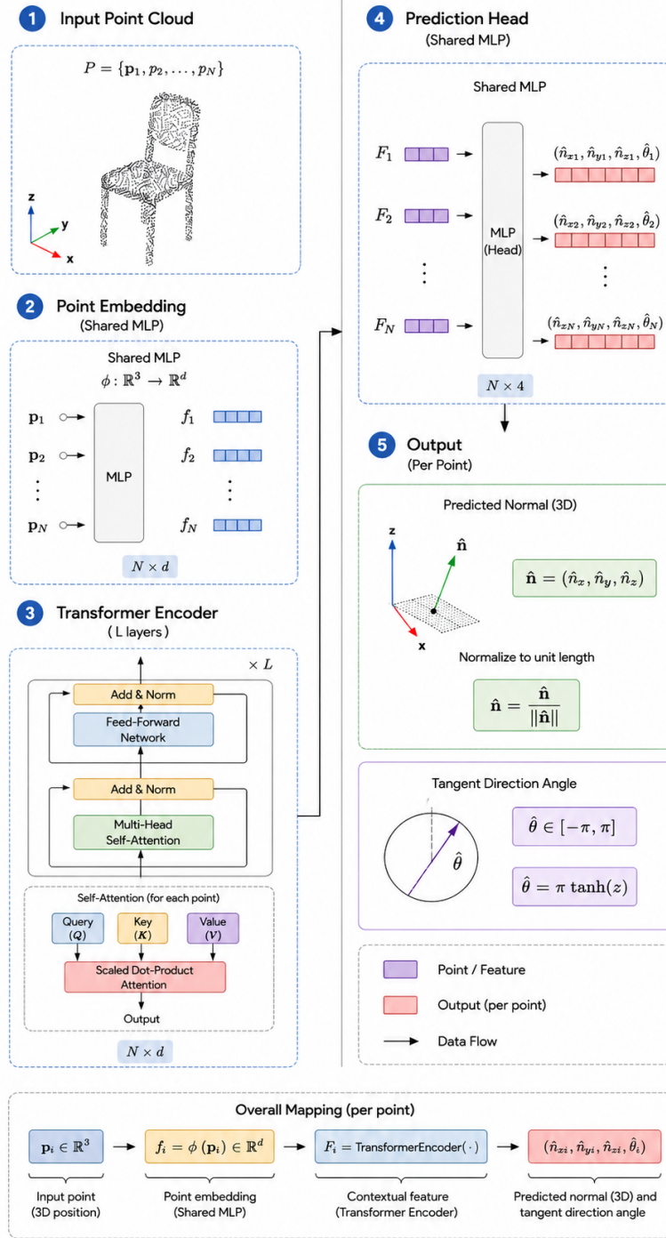
Figure 3.4: Pipeline of the proposed Transformer-based point cloud network. Input points are embedded into feature vectors, processed by stacked Transformer encoder layers, and decoded by a prediction head to predict a unit surface normal and tangent direction angle for every point.
