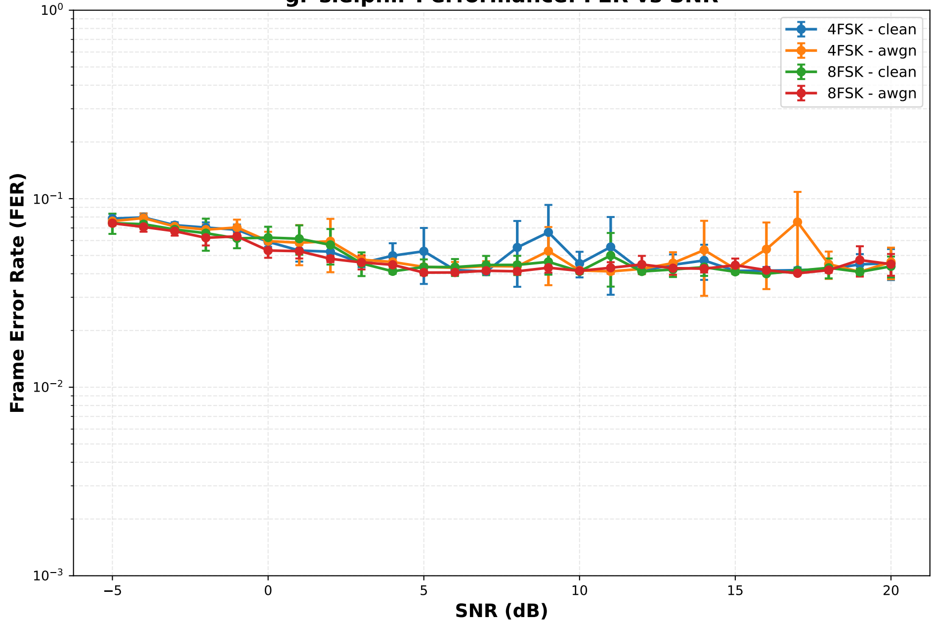
gr-sleipnir Performance: FER vs SNR
