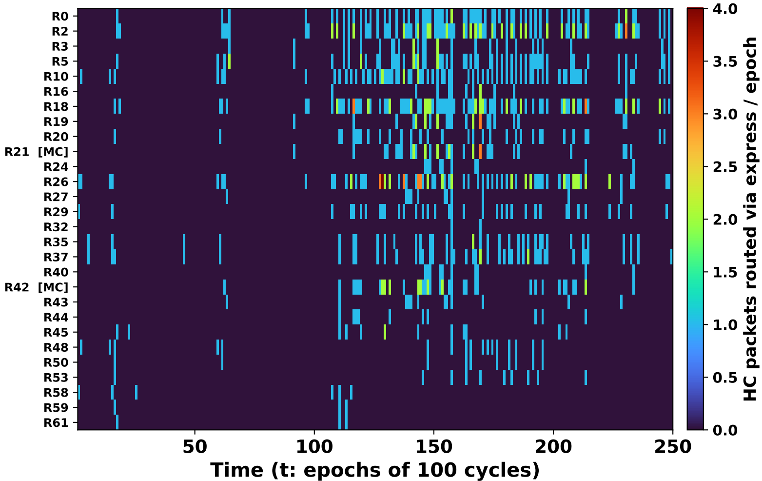
Mesh router (Express link)
