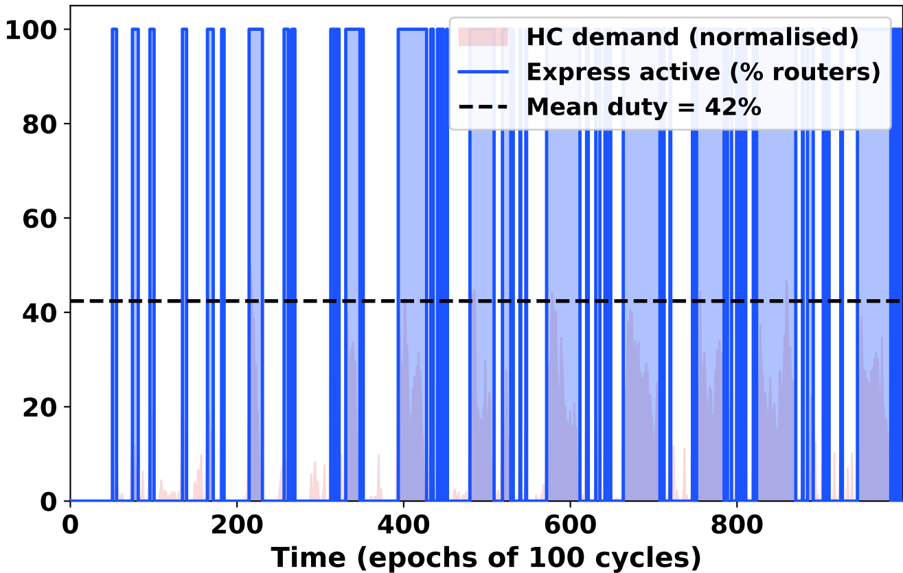
Express-link activity (% of routers ON)
