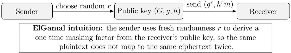
Figure 2: High-level ElGamal encryption flow.
