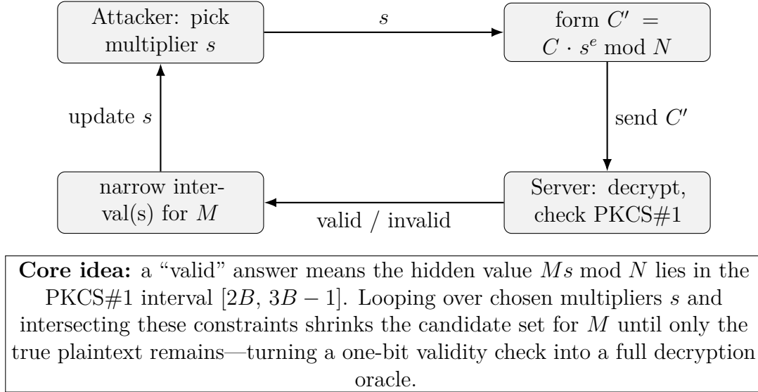
Figure 6: Bleichenbacher’s attack is an adaptive feedback loop: each oracle bit narrows the interval that must contain the plaintext.
