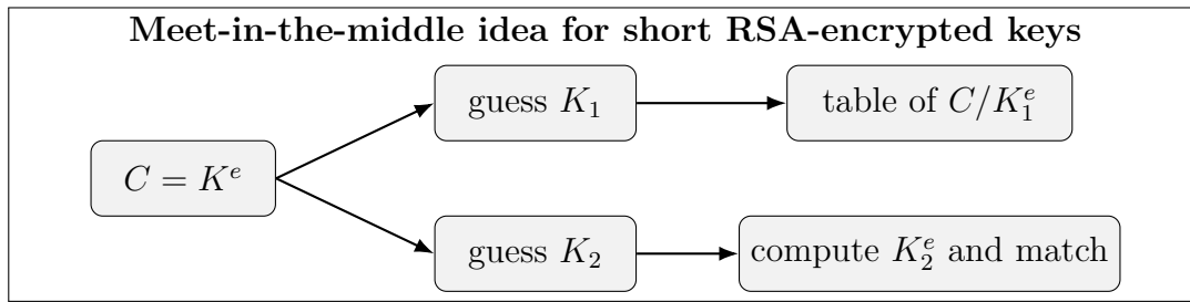
Figure 4: A structured plaintext space can make textbook RSA vulnerable to faster-than-brute-force search.
