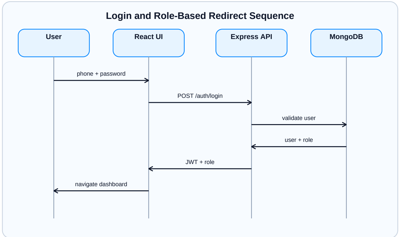
Figure: Login Sequence Diagram for the HealHub MERN stack application.
