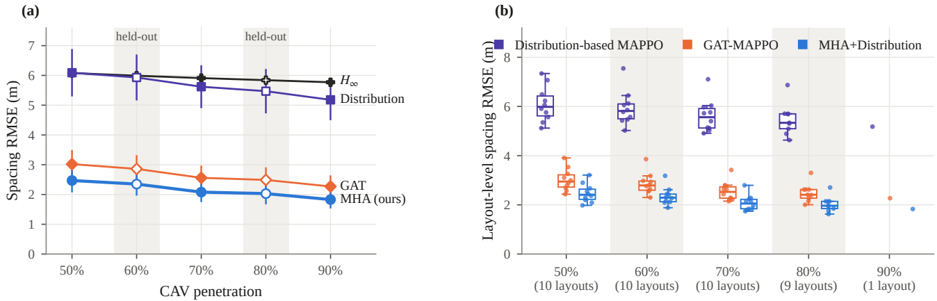
FIGURE 6. Generalization across CAV penetration and vehicle ordering at 30% Bernoulli loss. (a) Layout-averaged spacing RMSE (mean and 95% confidence interval over five seeds); open markers and shaded columns denote the held-out 60% and 80% rates. (b) Layout-level spacing RMSE (seed mean per layout) over the 10/10/10/9/1 evaluated layouts; boxes show the median and interquartile range.
