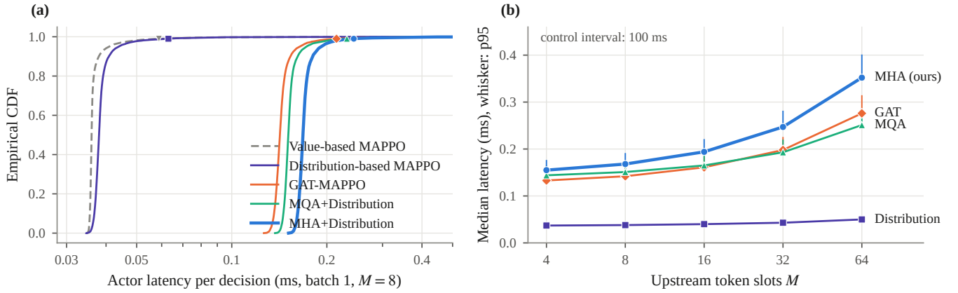
FIGURE 17. Actor inference cost on a single CPU thread with batch size one. (a) Empirical distribution of the latency per decision at M = 8 over 10,000 timed forward passes (markers: 99th percentile). (b) Median latency (whiskers: 95th percentile) versus the number of upstream token slots M .
