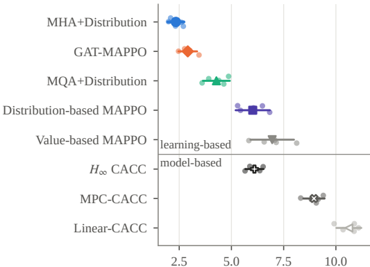
(a) Spacing RMSE (m), lower is better
