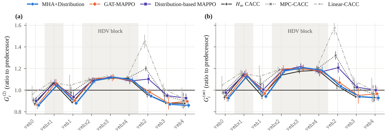
FIGURE 15. Finite-window (a) L_2 and (b) L_\infty disturbance-amplification ratios versus vehicle position under the bounded lead-vehicle pulse at the anchor condition (mean and 95% confidence interval over five seeds; shaded positions are HDVs; the horizontal line marks non-amplification). Value-based MAPPO and MQA+Distribution are omitted for readability and are reported in Table 9.
