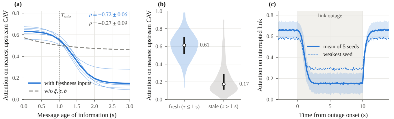
FIGURE 12. Repeated attention-freshness analysis over five seeds. (a) Head-averaged attention on the nearest upstream CAV token versus its message age (thin: individual seeds; thick: mean), with and without the explicit freshness inputs, and the seed-level Spearman correlation. (b) Attention on the nearest upstream CAV token for fresh and stale messages (violin: distribution; bar: interquartile range; circle: median). (c) Event-aligned attention on the interrupted link around a 10-s outage (mean and 95% confidence interval; dashed: weakest seed).
