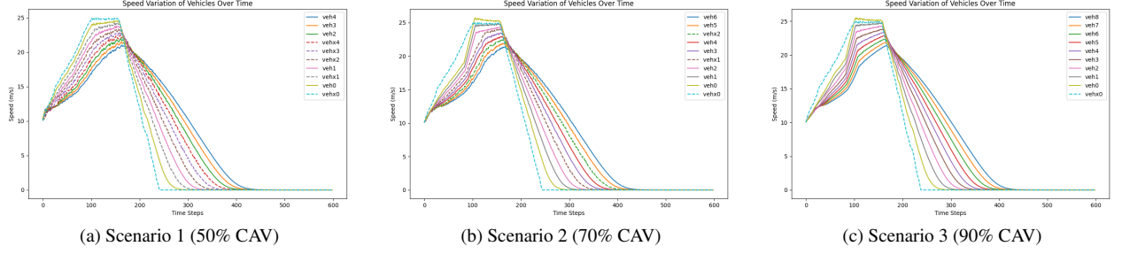
FIGURE 13. Velocity profiles under varying penetration rates during sudden lead vehicle deceleration.
