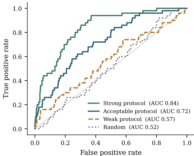
ROC behaviour across protocol quality
