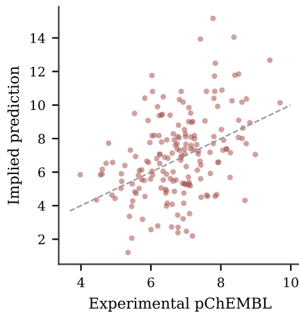
Same model vs reality R^2 = 0.16
