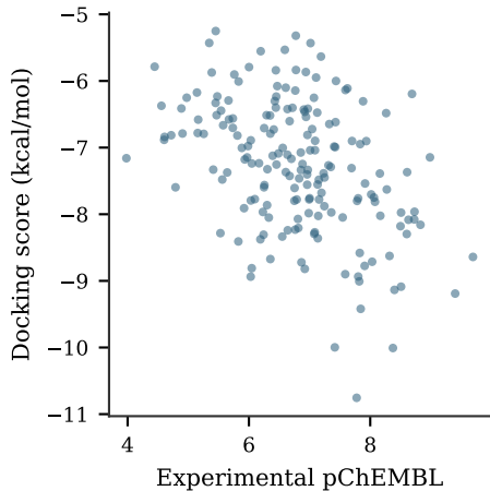
Docking vs experiment r = -0.42
