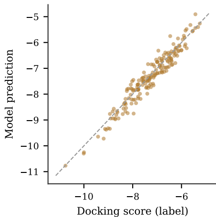
Trained on docking scores R^2 = 0.93 vs the WRONG target
