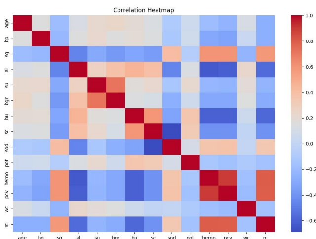
Fig. 1: Correlation Heatmap
