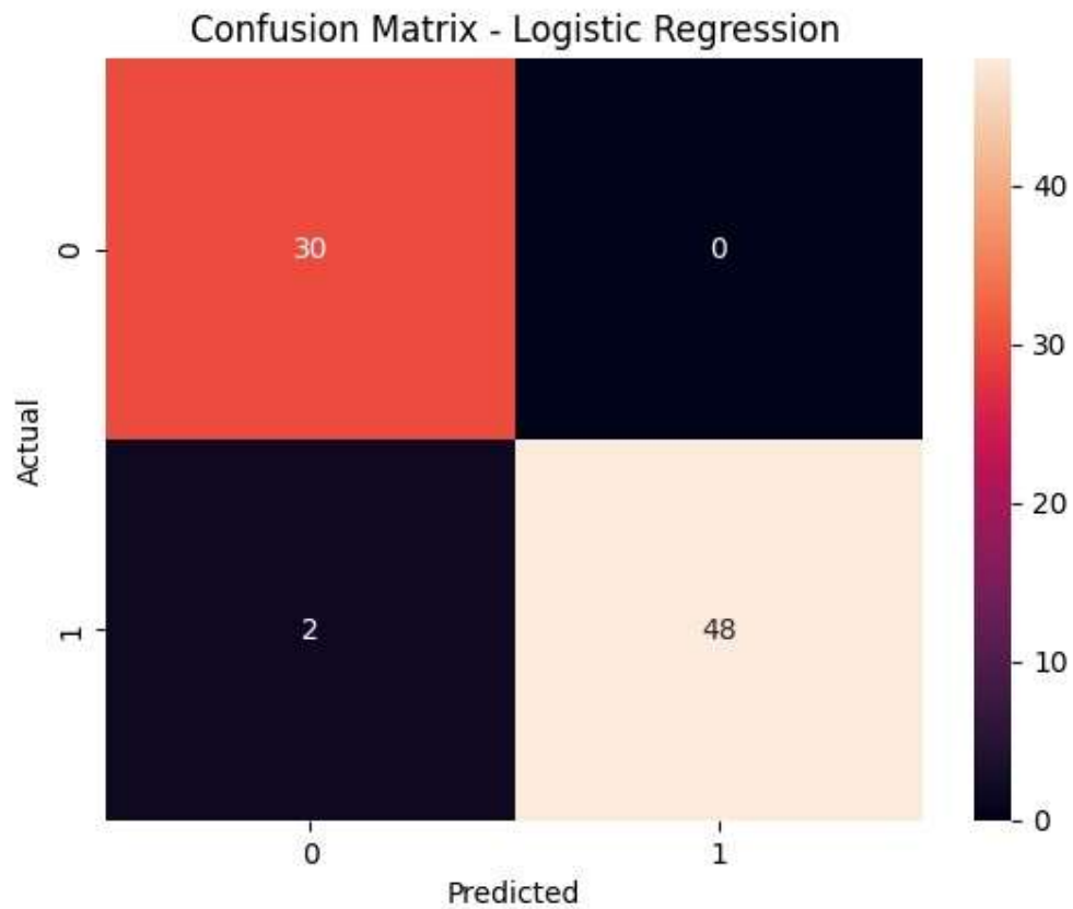
Fig. 9: Confusion Matrix — Logistic Regression
