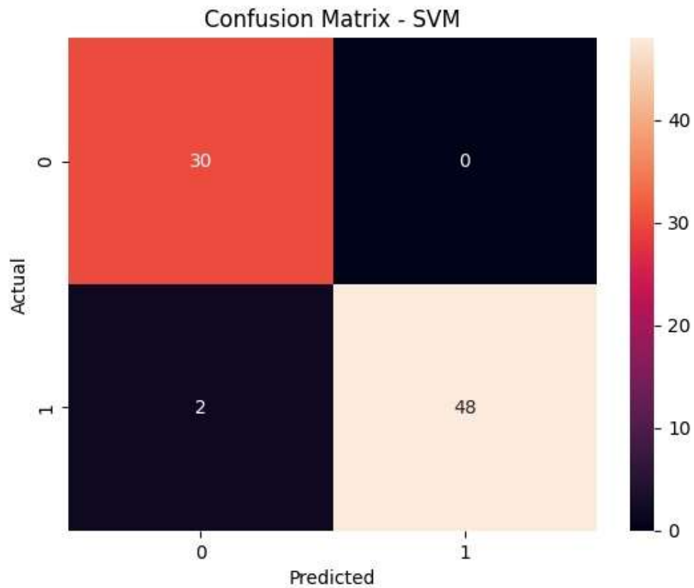
Fig. 15: Confusion Matrix — SVM
