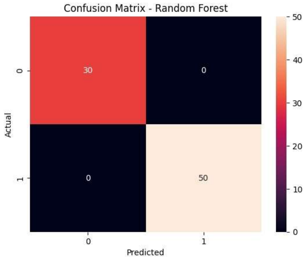
Fig. 13: Confusion Matrix — Random Forest
