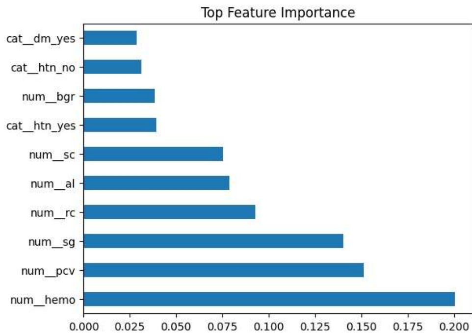
Fig. 18: Top Feature Importance Graph
