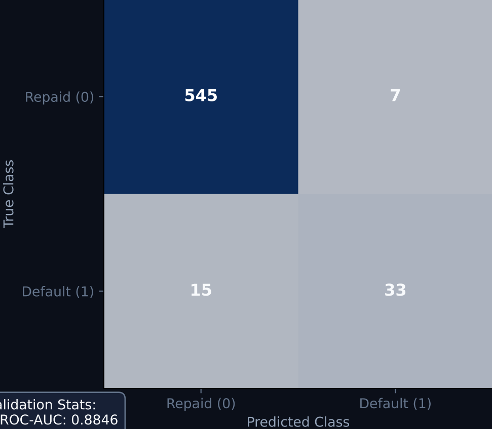
Confusion Matrix
