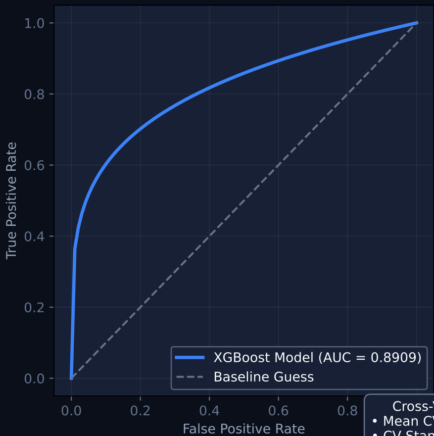
ROC Curve (Holdout Set)
