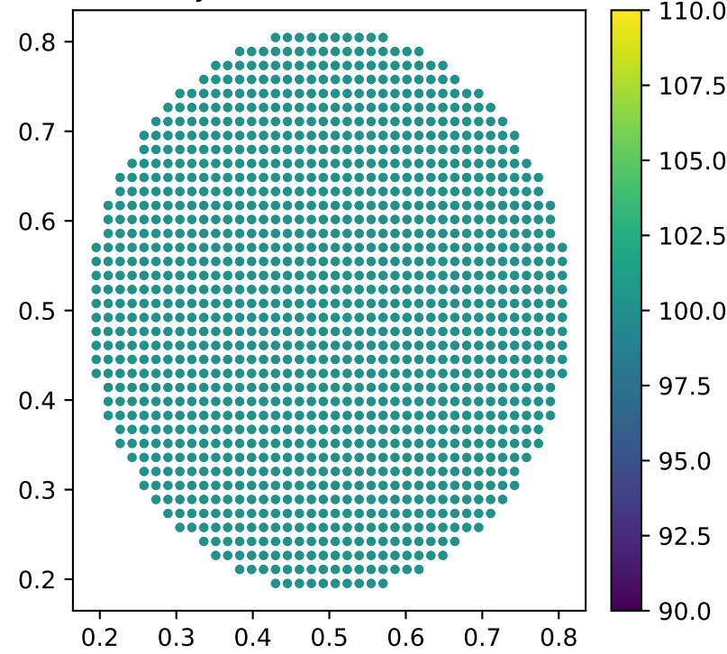
xy central slice: T [K]
