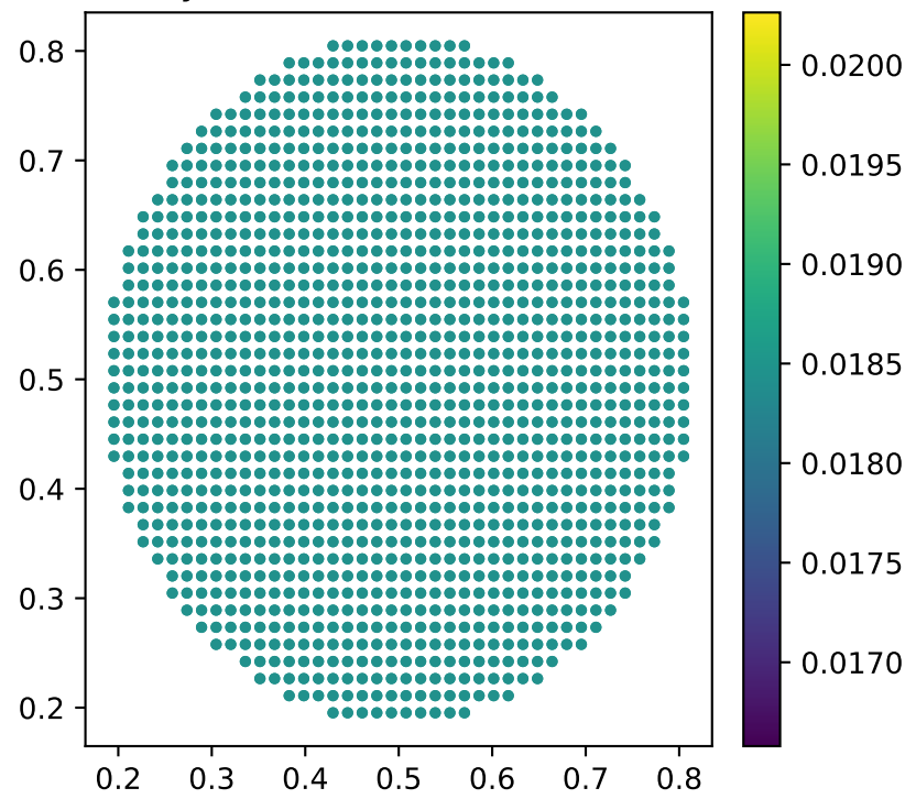
xy central slice: nHI [cm -3 ]
