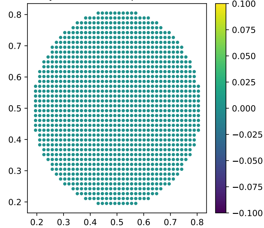
xy central slice: speed [cm/s]
