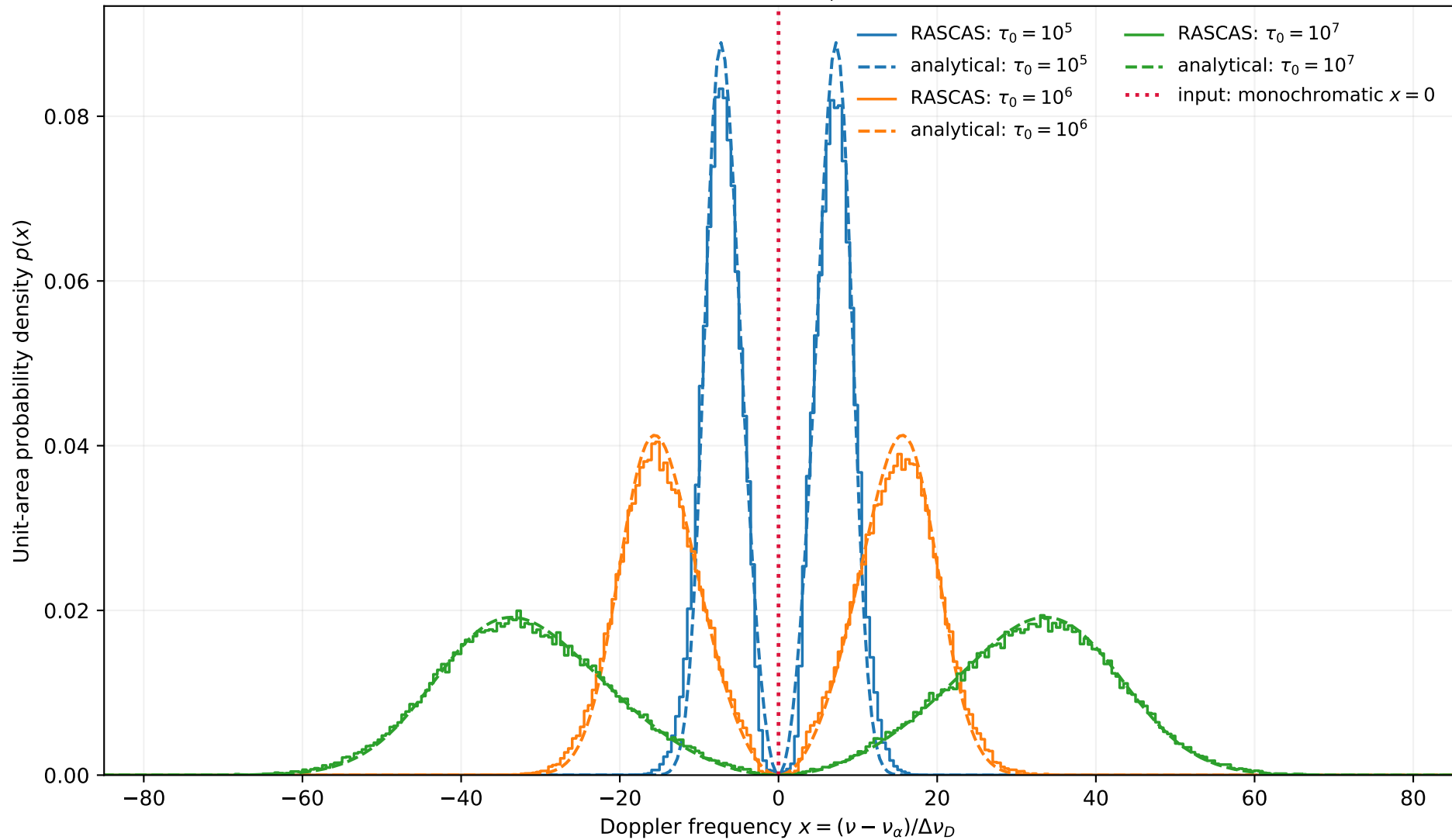
Existing static-sphere spectra: N_\gamma = 10^5 per optical depth
