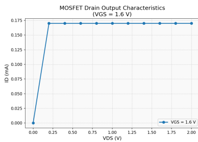
(a) V_{GS} = 1.6\text{ V}
