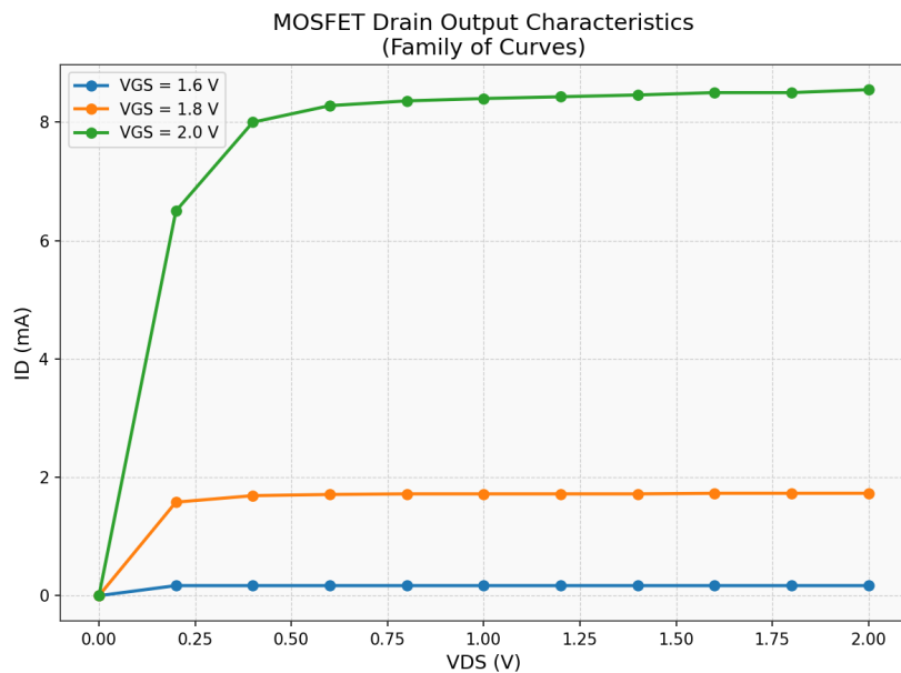
Figure 4: Combined Family of Experimental Output Characteristic Curves ( I_D vs V_{DS} ).
