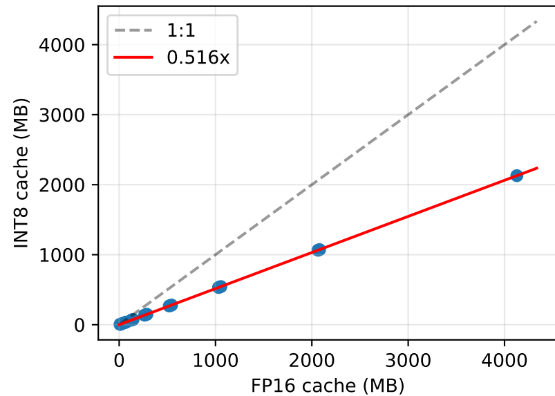
Cache memory: INT8 vs FP16
