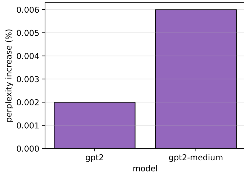
INT8 quality cost (WikiText-2)
