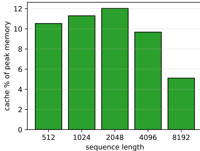
Cache is a small share of peak
