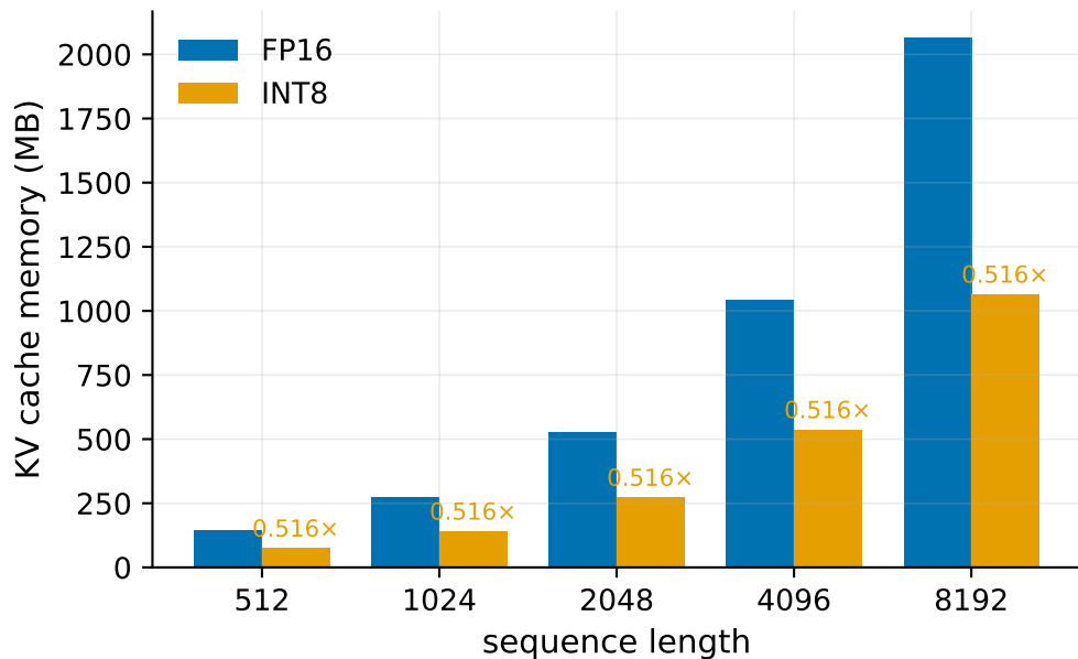
(a) INT8 cache \approx 0.516\times FP16, constant
