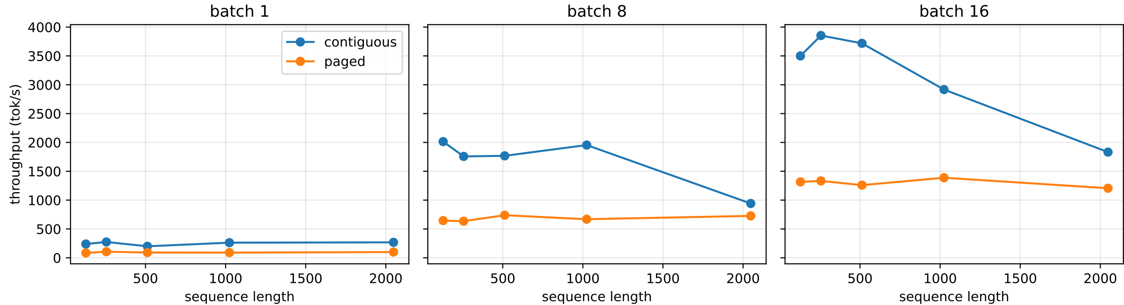
Contiguous vs paged throughput (paged indirection overhead)
