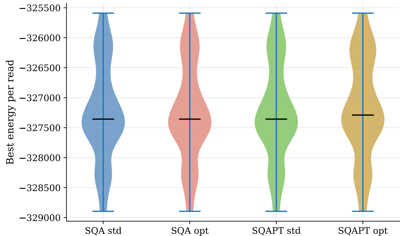
Planted Partition (n=512)
