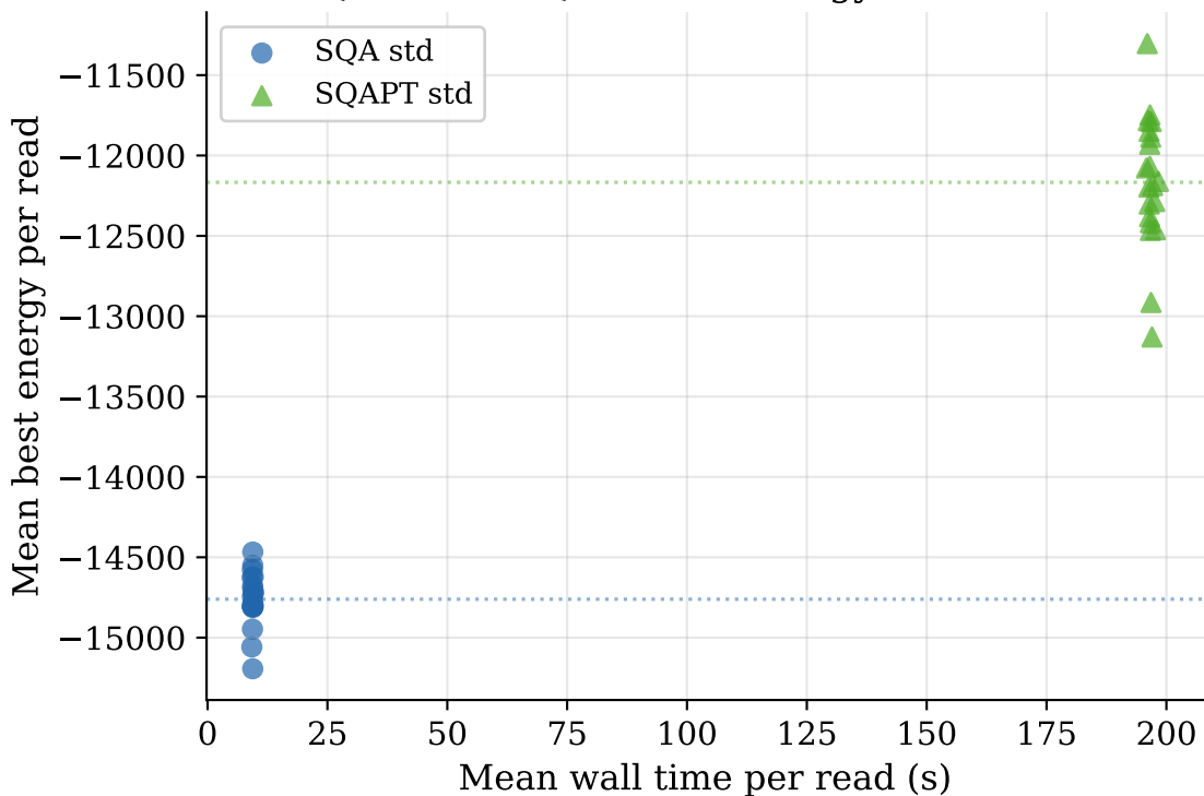
SK Spin Glass (n=256) SQA-std vs SQAPT-std: energy vs wall time
