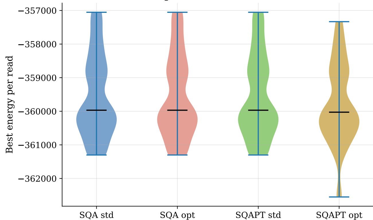
Weighted MAX-CUT (n=512)
