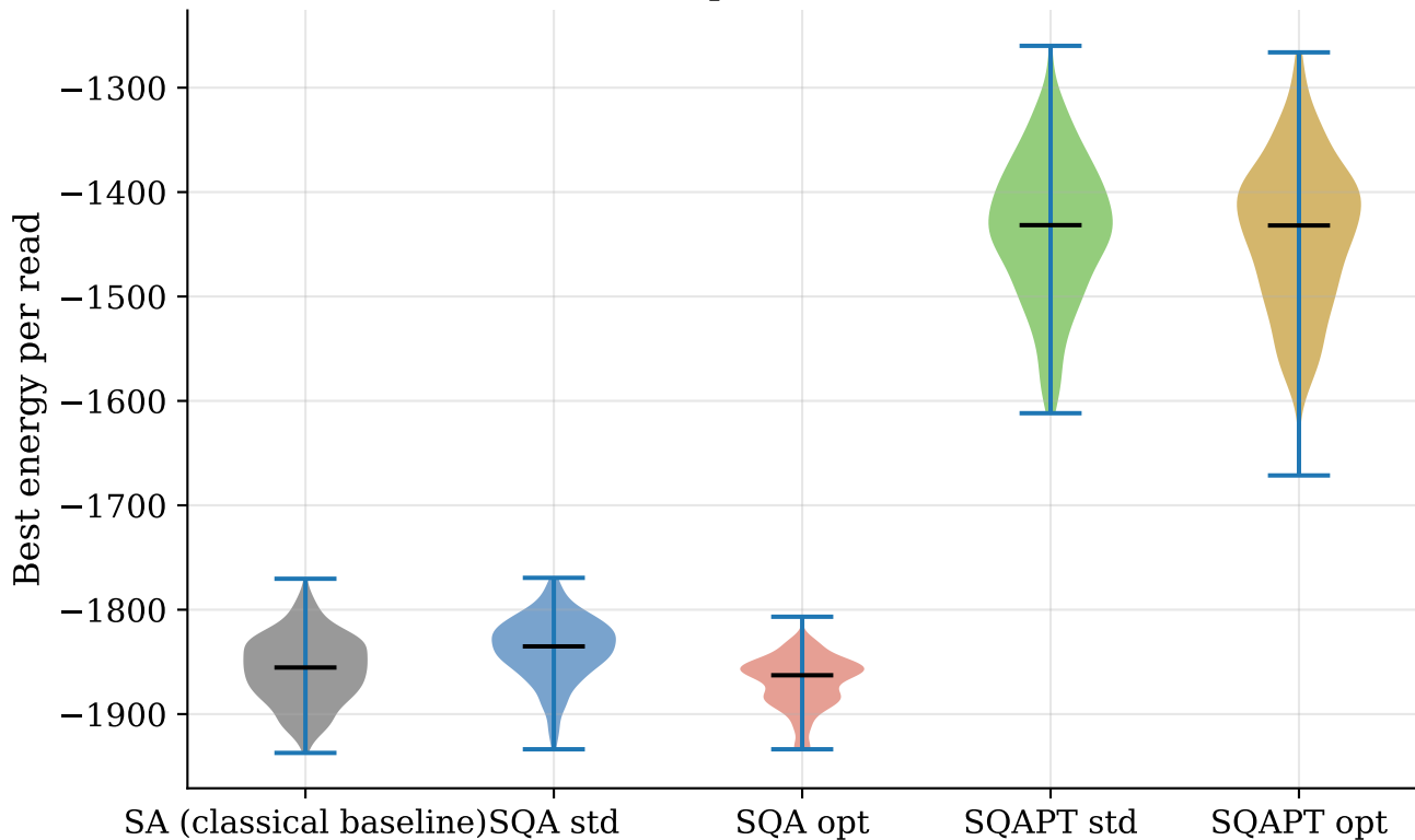
3D EA Spin Glass (n=216)
