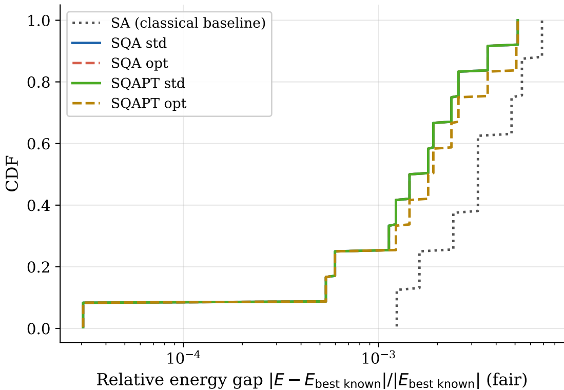
Planted Partition (n=512)
