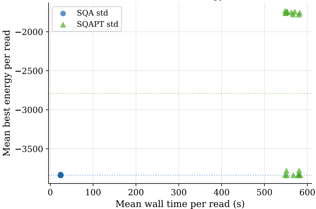
3-Regular MAX-CUT (n=512) SQA-std vs SQAPT-std: energy vs wall time
