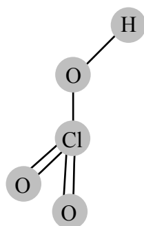
The structures of oxoacids of chlorine
