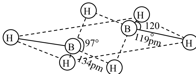
The structure of diborane, B_2H_6
