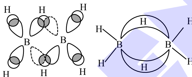
Figure: Bonding in diborane.
