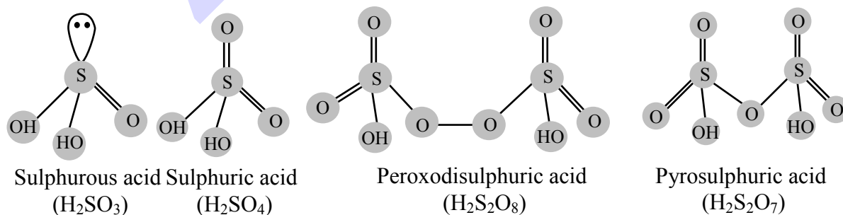
Structures of some important oxoacids of sulphur
