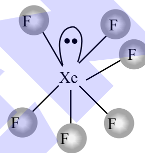
(c) Distorted octahedral
