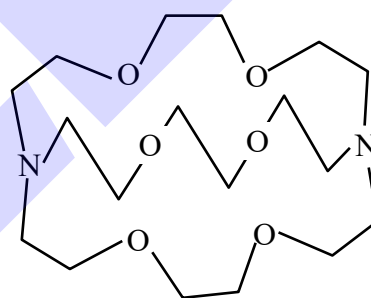
Cryptand-222
