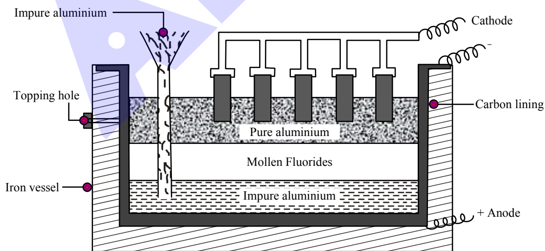
(Hoop's process) Pure Al (99.98% pure)
